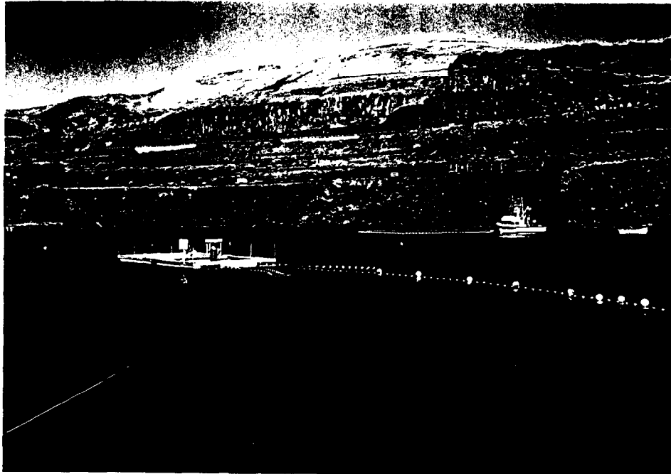
Plate 3.1 The Merwin traps' anchoring scheme. U of W Purse Seiner shown in background.
