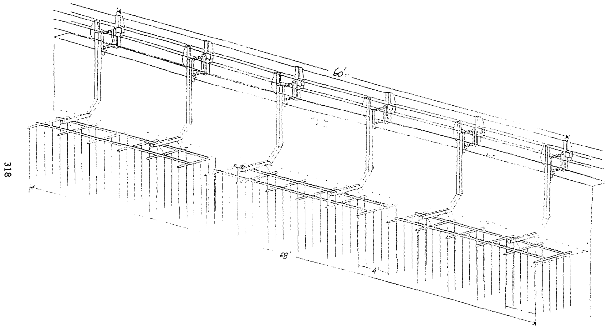
Appendix Figure E-1. View of three wingwall arrays used for electrofishing northern squawfish at Bonneville Dam First Powerhouse.
